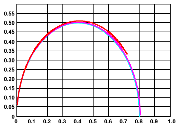
FIGURE 28. NORMALIZED RMS INPUT CURRENT
